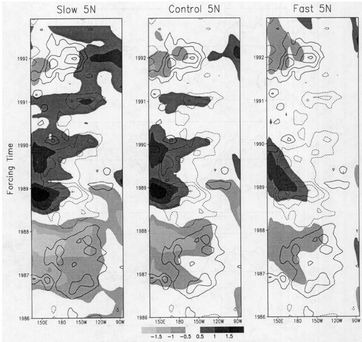
FIG. 14. Time series of heat content anomalies at 5°N (°C, shaded) as obtained in the Slow experiment, in which the wind stress evolution was slowed down by a factor of 2 (left), Control (center), and the Fast experiment, in which the forcing was speeded up by a factor of 3 (right). The superimposed contours in each panel are the equatorial wind stress anomalies, contour interval 0.1 dyn, zero contour suppressed (cf. Fig. 4b).
