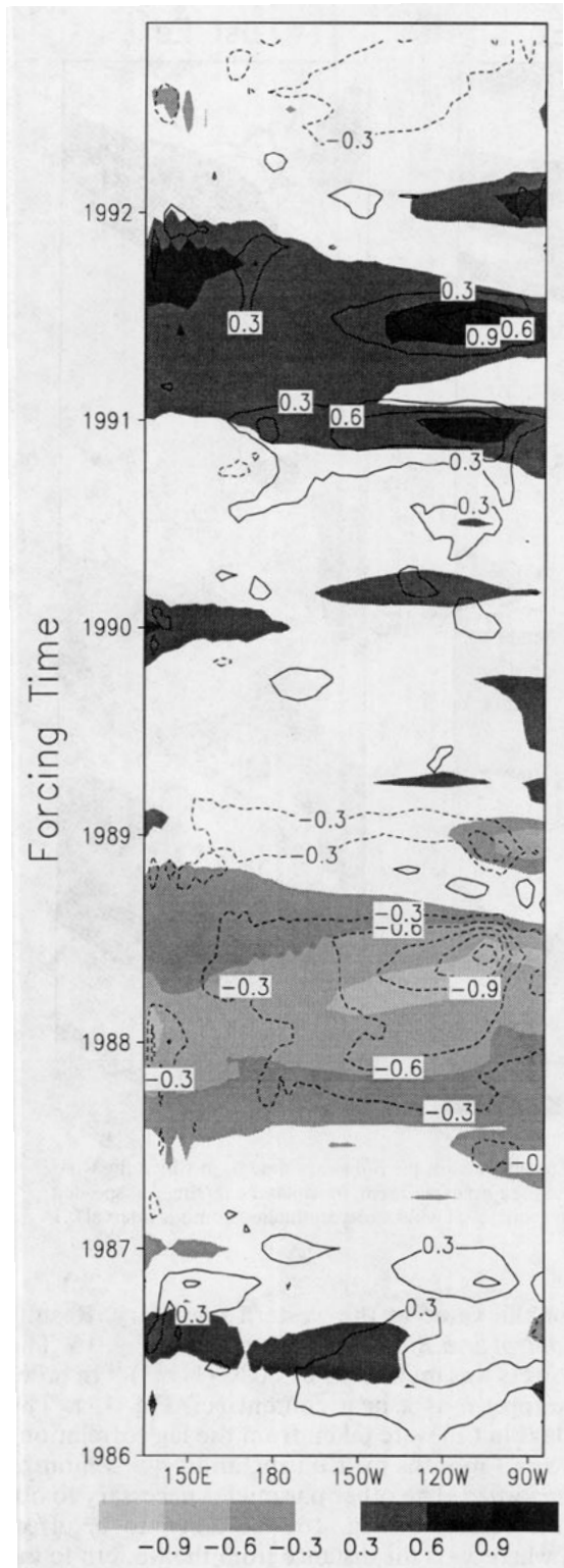
FIG. 12. Difference (one-half of Control minus Backward ) equatorial heat content anomalies ( ^{\circ}\text{C} , shaded). Difference (one-half of Control minus Backward ) equatorial SST anomalies (contours, cf. Fig. 4a). Contour interval 0.3^{\circ}\text{C} , zero contour suppressed.
