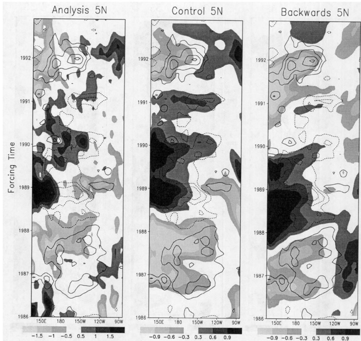
FIG. 10. Time series of heat content anomalies at 5°N (°C, shaded) as obtained by the NMC Pacific Ocean retrospective data-assimilation system (left, Lectma and Ji 1989), Control (center), and Backward (right). The superimposed contours in each panel are the equatorial wind stress anomalies (cf. Fig. 4b), contour interval 0.1 dyn, zero contour suppressed. A nine-point space-time smoother has been applied to all of the plotted fields.
