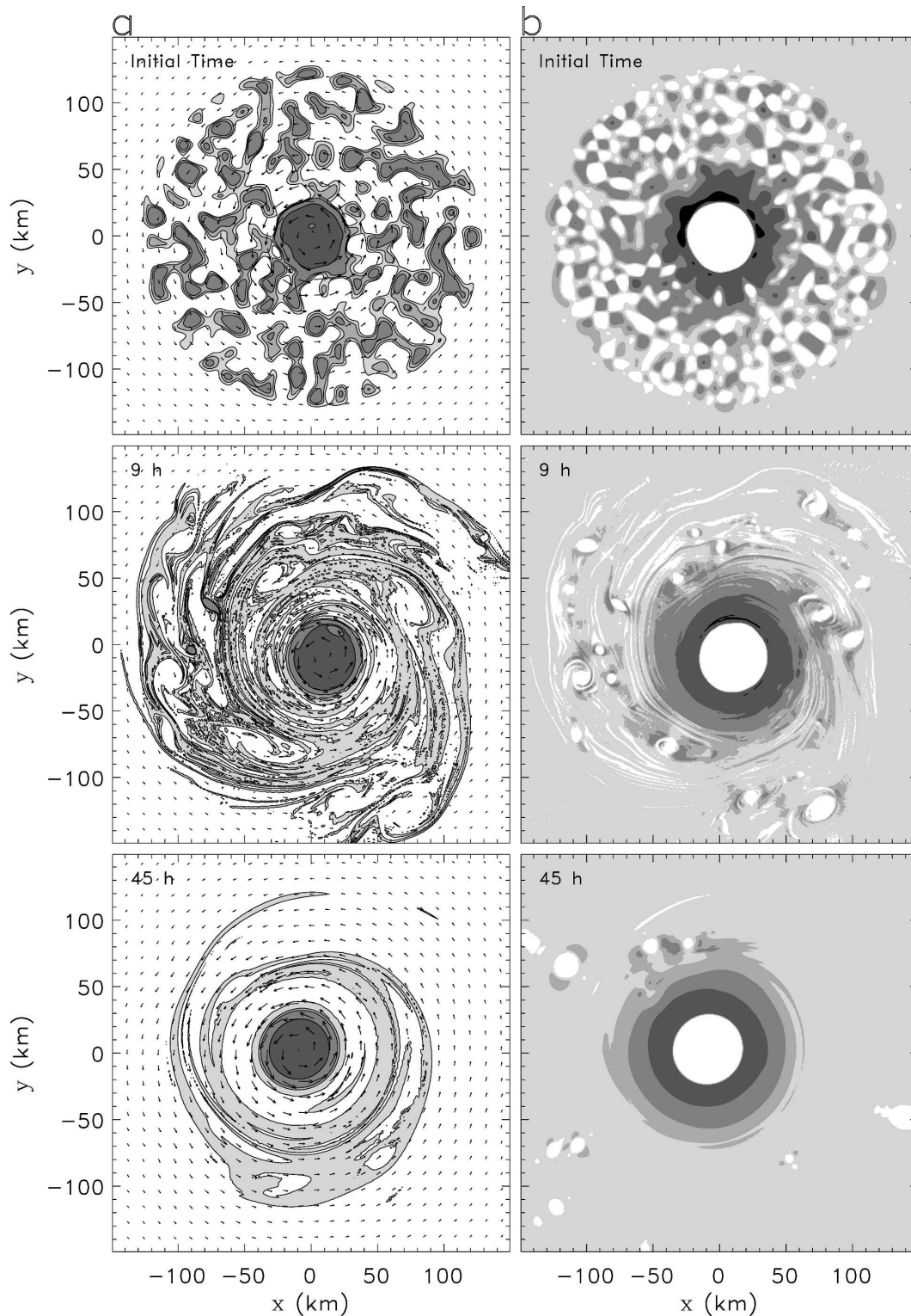
FIG. 7. (a) Vorticity contour plots and horizontal wind vectors. The contours are 1 \times 10^{-4} , 5 \times 10^{-4} , 10 \times 10^{-4} , and 50 \times 10^{-4} \text{ s}^{-1} . Darker shading denotes higher vorticity. (b) Corresponding filamentation times for the panels to the left. Shaded regions are separated by filamentation times of 45, 30, 15, and 7.5 min, with darker shadings representing the smallest times. The model domain is 600 \text{ km} \times 600 \text{ km} , but only the inner 300 \text{ km} \times 300 \text{ km} is plotted.
