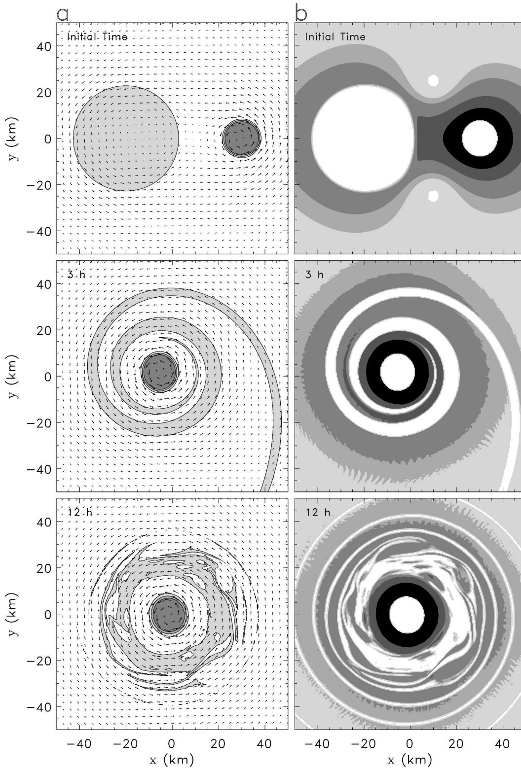
FIG. 6. (a) Vorticity contour plots and horizontal wind vectors for the binary interaction experiment are shown in the left three panels. The contours are 10 \times 10^{-4} , 50 \times 10^{-4} , and 100 \times 10^{-4} \text{ s}^{-1} , with darker shading denoting higher vorticity. (b) Corresponding filamentation times for the panels to the left. The shaded regions are separated by filamentation times of 45, 30, 15, and 7.5 min, with darker shadings representing the smallest times. The model domain is 200 \text{ km} \times 200 \text{ km} but only the inner 100 \text{ km} \times 100 \text{ km} is plotted.
