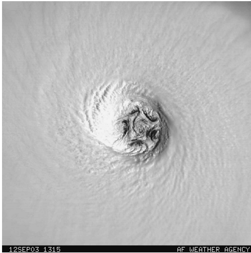
FIG. 10. DMSP ( FI5 ) visible image of Hurricane Isabel on 1315 UTC 12 Sep 2003. At 0900 UTC 12 Sep, the MSLP was 936 hPa. At 1500 UTC 12 Sep, the MSLP was 924 hPa. The approximate dimensions of the figure are 200 km \times 200 km.
