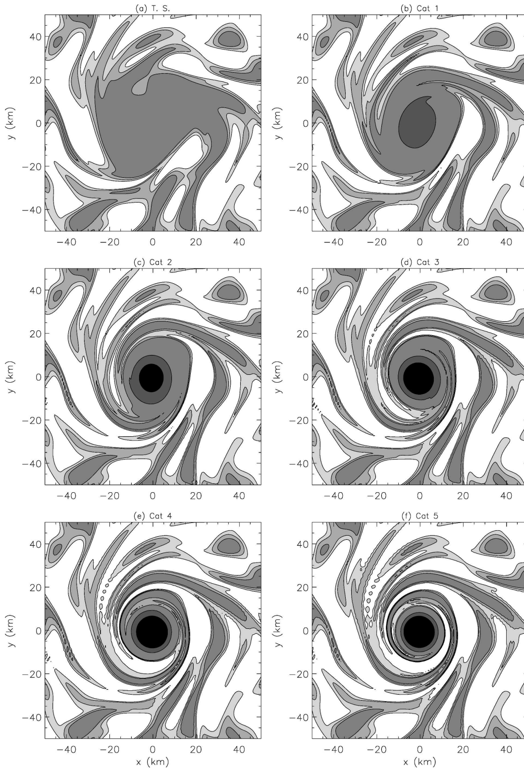
FIG. 5. Barotropic model results at t = 30 min for the six Gaussian vortices with a superimposed turbulent field. Vorticity is plotted for (a) b = 20 km (tropical storm), (b) b = 13 km (category 1 tropical cyclone), (c) b = 10.2 km (category 2), (d) b = 8.5 km (category 3), (e) b = 7.4 km (category 4), and (f) b = 6.3 km (category 5). Shaded regions are separated by the vorticity contours 1 \times 10^{-4} , 5 \times 10^{-4} , 10 \times 10^{-4} , 50 \times 10^{-4} , and 100 \times 10^{-4} \text{ s}^{-1} . The darker shading represents higher values of vorticity. The model domain encompasses 600 \text{ km} \times 600 \text{ km} , but only the inner 100 \text{ km} \times 100 \text{ km} is displayed.
