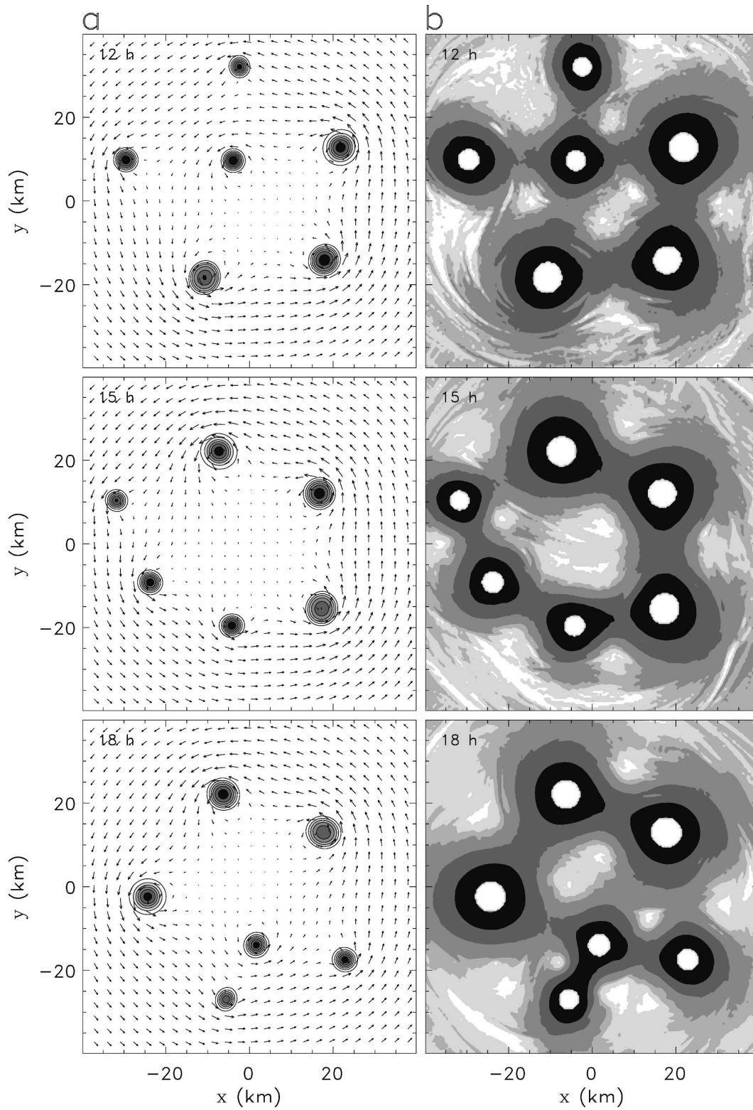
FIG. 9. (a) Vorticity contour plots and horizontal wind vectors for the second thin annular vorticity ring experiment. The contours begin at 5 \times 10^{-3} \text{ s}^{-1} and are incremented by 5 \times 10^{-3} \text{ s}^{-1} . Darker shading denotes higher vorticity. (b) Corresponding filamentation times for the panels to the left. Shaded regions are separated by filamentation times of 45, 30, 15, and 7.5 min, with darker shadings representing the smallest times. The model domain is 200 \text{ km} \times 200 \text{ km} but only the inner 80 \text{ km} \times 80 \text{ km} is plotted.
