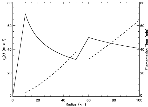
FIG. 3. An idealized vortex with a secondary eyewall. The solid curve is v_{\theta}(r) as given by (17), and the dashed curve is the filamentation time \tau_{\text{fil}}(r) , as given by (18). The filamentation time is plotted only in the regions, where S_1^2 + S_2^2 - \zeta^2 > 0 .
