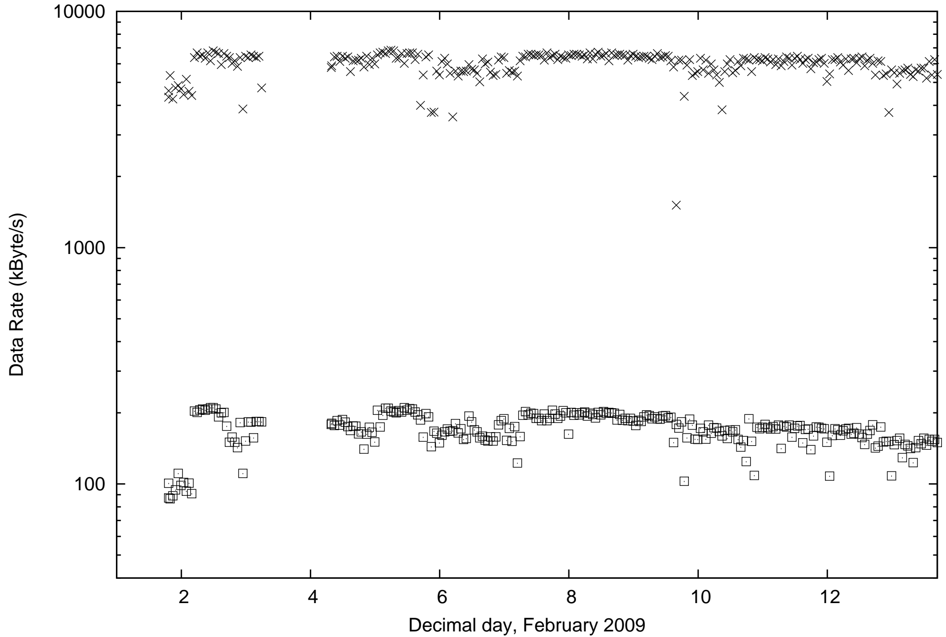
Transferring a 10 MByte file (x), and 100 kByte (o): feynman-to-rainbow
