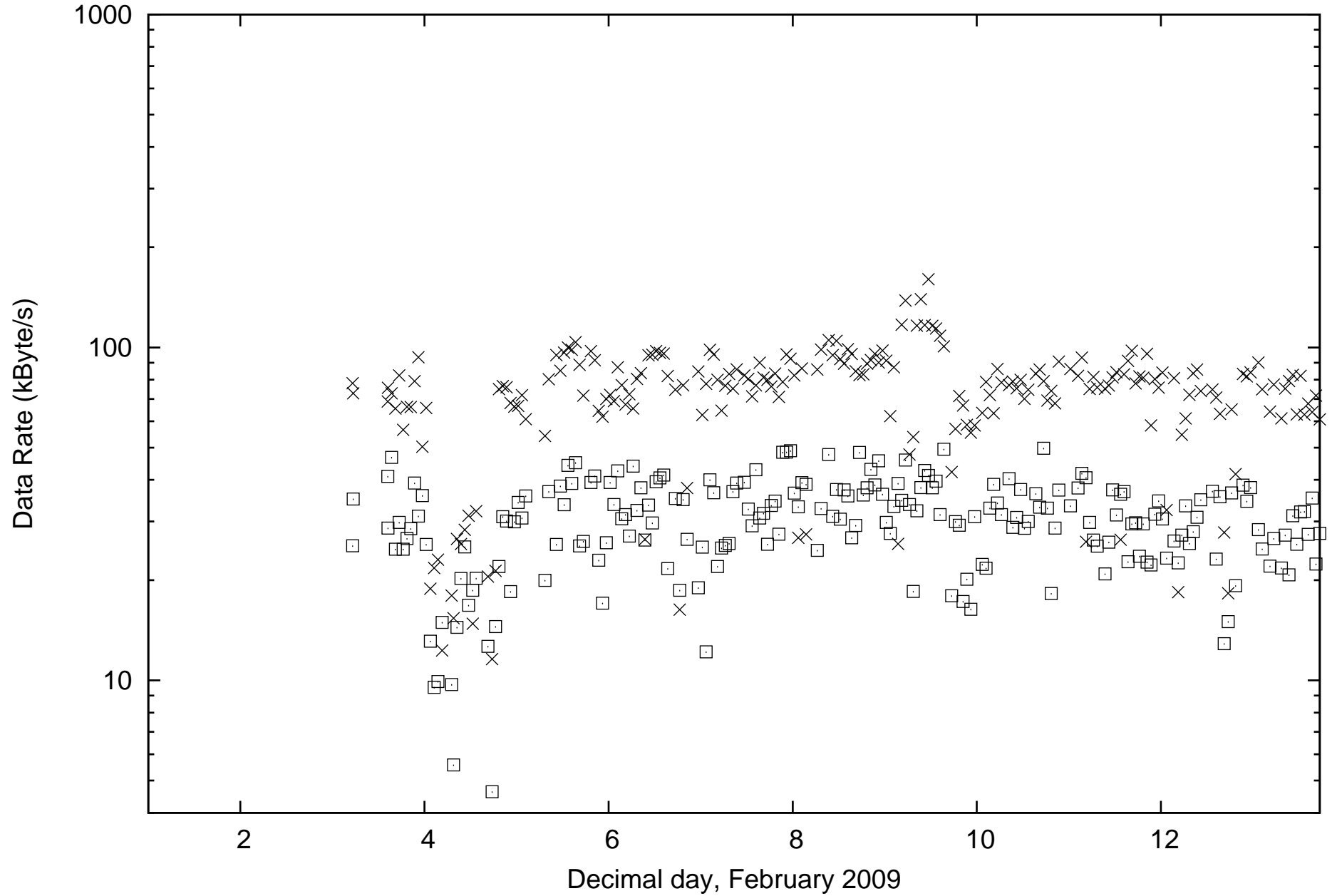
Transferring a 10 MByte file (x), and 100 kByte (o): feynman-to-cesium
