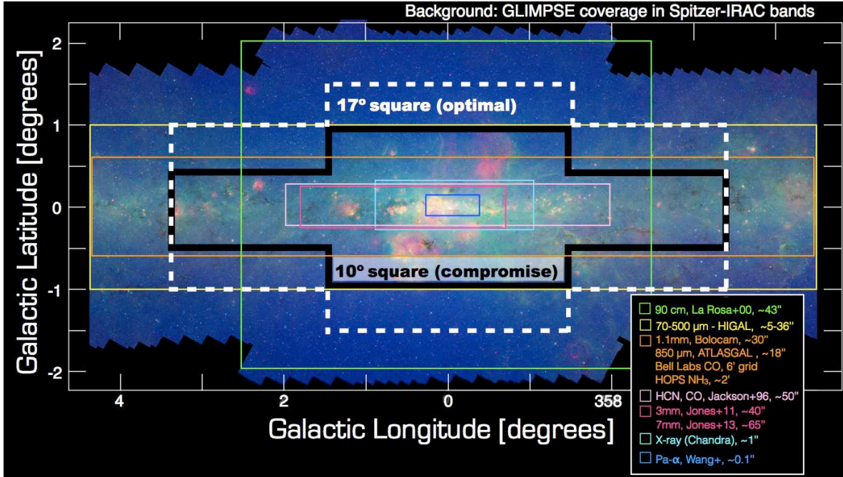
Fig. 3.— Recommended coverage areas for a deep VLASS mosaic of the Galactic center in C band ( 4\text{--}8 GHz) continuum, recombination lines, \text{H}_2\text{CO} , and \text{CH}_3\text{OH} masers, compared to coverage of existing surveys. The diffuse red emission at l = 359.5, b = 0.5 enclosed in a shell of green emission is the GC lobe (Sofue 1985), suggested to be an outflow from the Galaxy’s nucleus.
